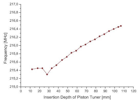
Figure 6: Frequency shift due to the piston tuner.
