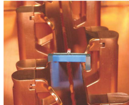
Figure 5: Perturbation capacitor used to detune each cell of the RFQ.
